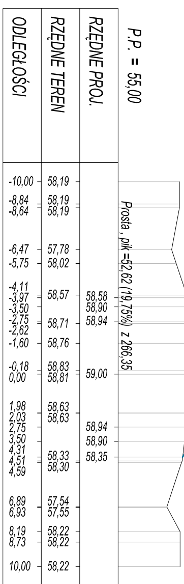
PK = 2+919,46 Skala 1:200/200
