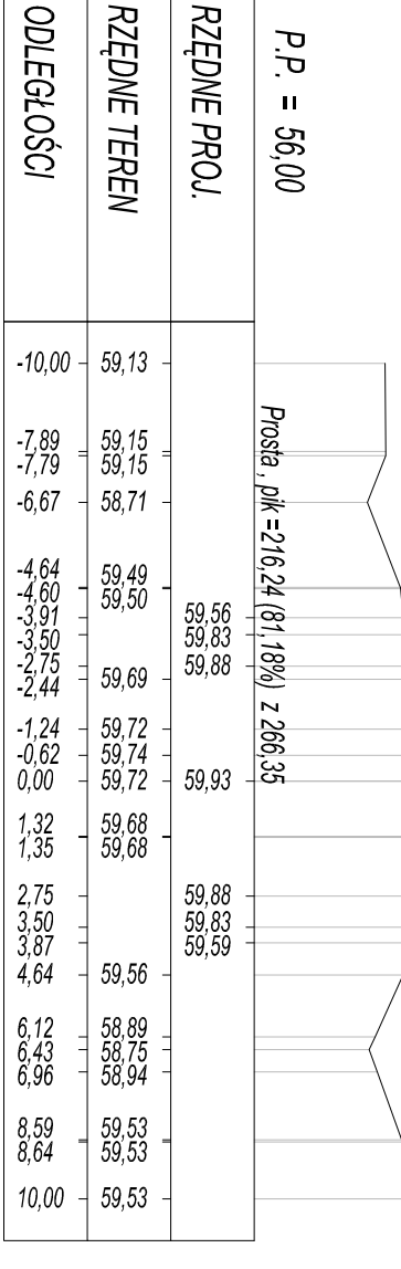
PK = 2+986,75 Skala 1:200/200
