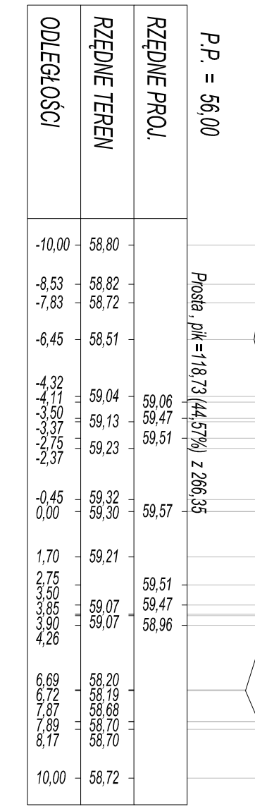
PK = 2+934,93 Skala 1:200/200
