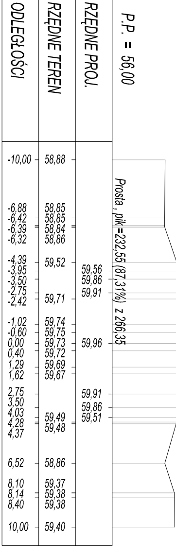
PK = 2+936,75 Skala 1:200/200
