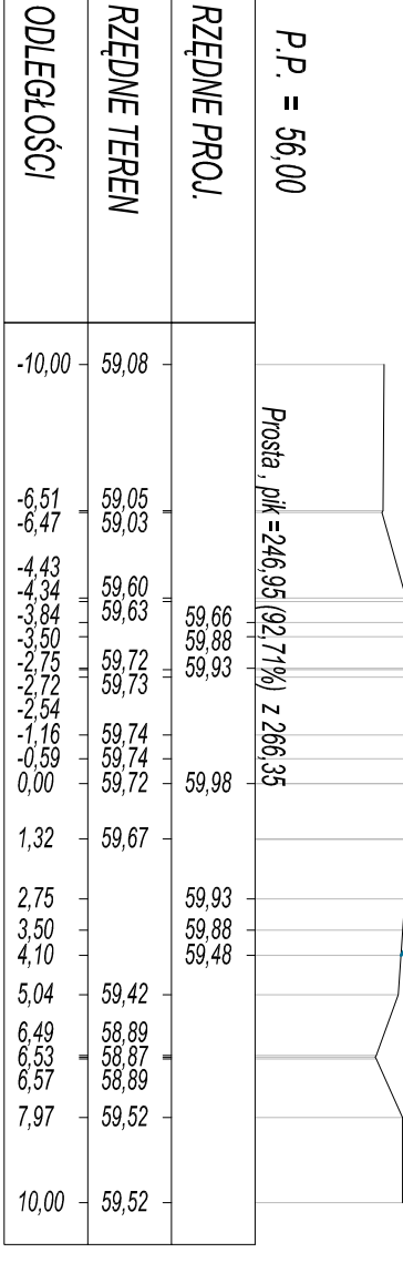
PK = 2+941,32 Skala 1:200/200
