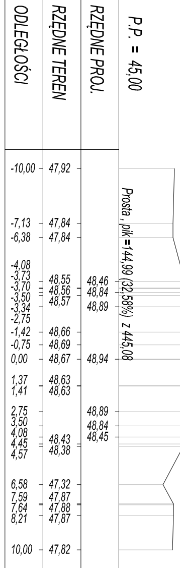
PK = 2+063,93 Skala 1:200/200
