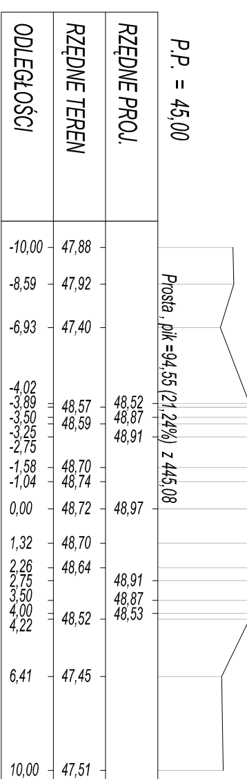
PK = 2+003,49 Skala 1:200/200
