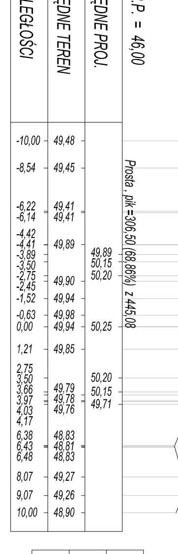
PK = 2+216,44 Skala 1:200/200
